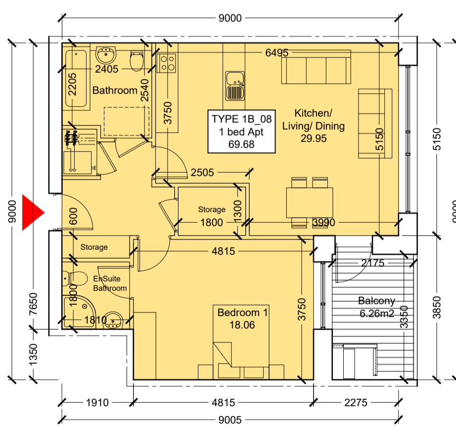
Type 1B_08 Scale 1:100
