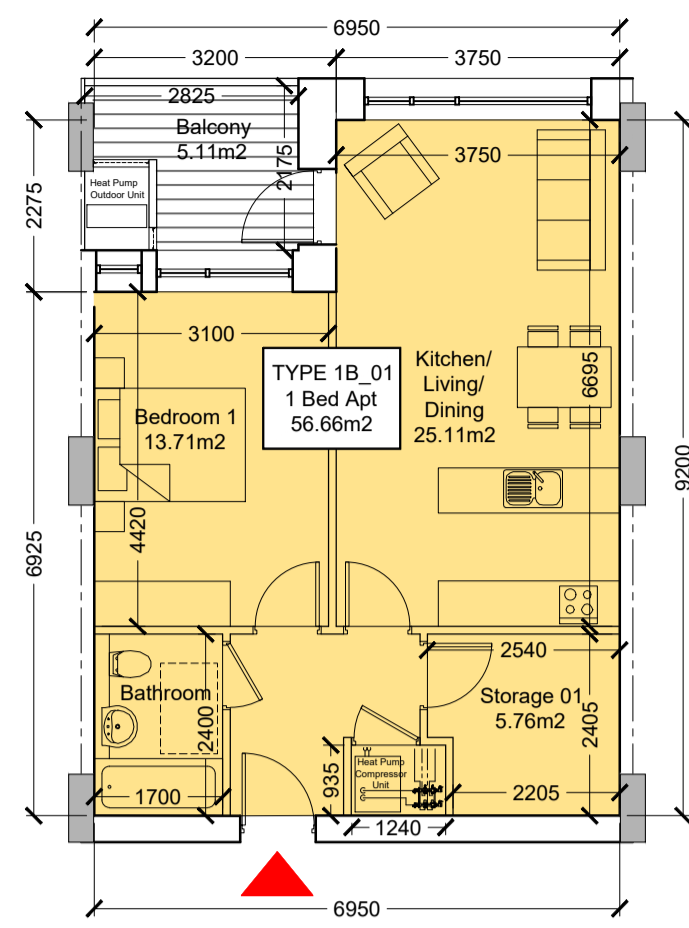
Type 1B_01 Scale 1:100
