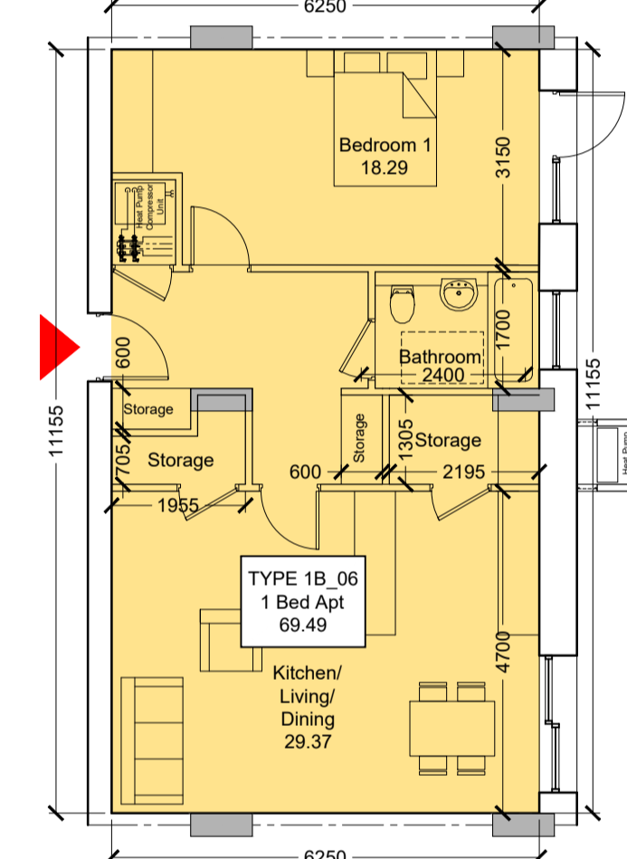
Type 1B_06 Scale 1:100
