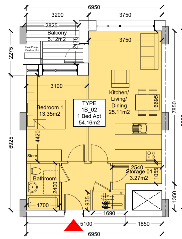
Type 1B_02 Scale 1:100
