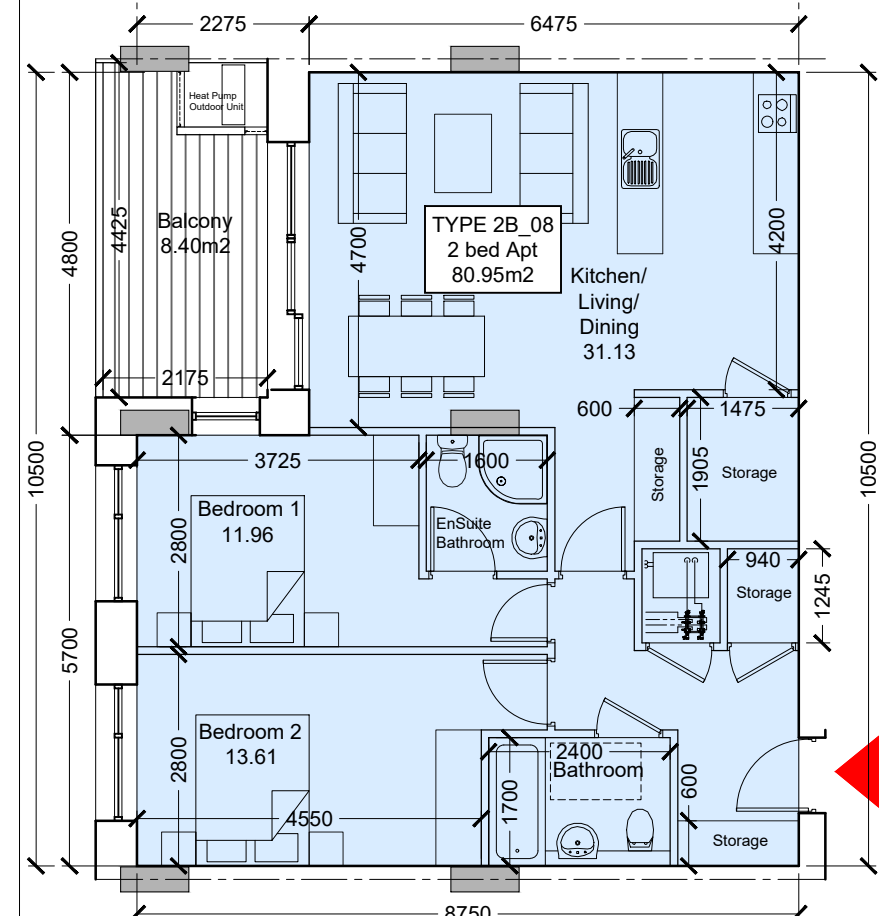
Type 2B_08 Scale 1:100
