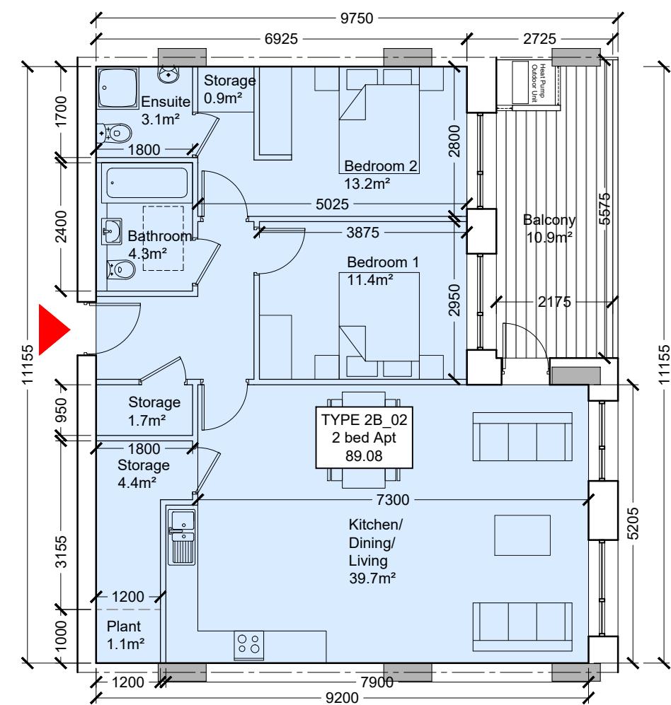
Type 2B_02 Scale 1:100
