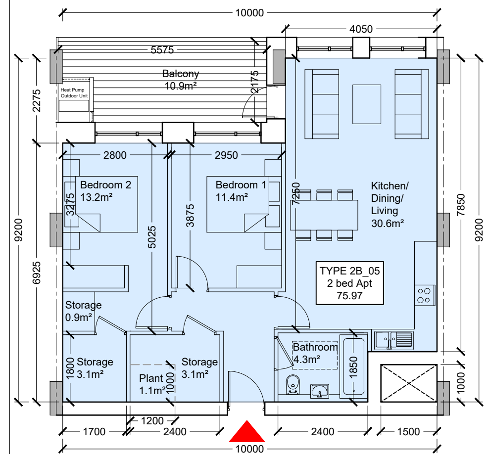
Type 2B_05 Scale 1:100
