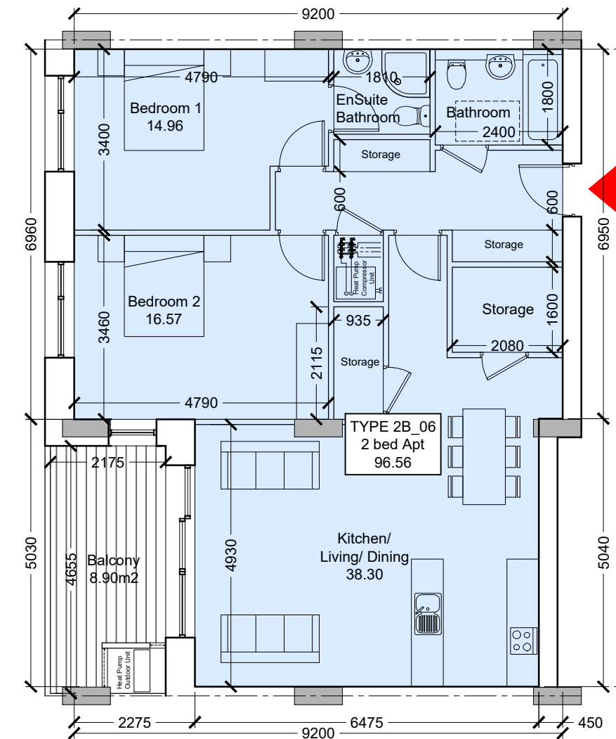
Type 2B_06 Scale 1:100
