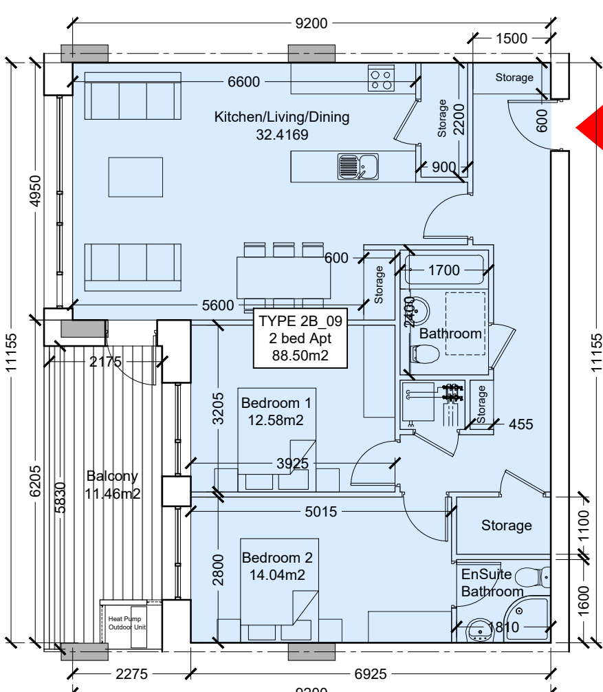
Type 2B_09 Scale 1:100
