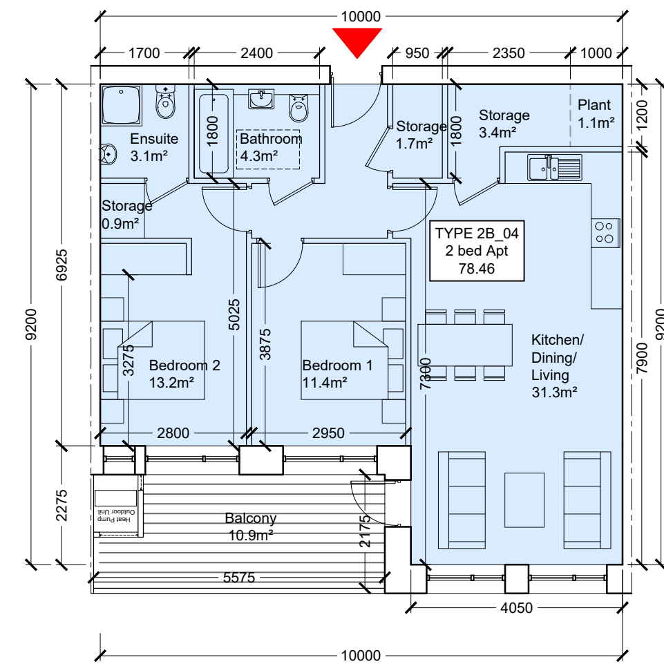
Type 2B_04 Scale 1:100
