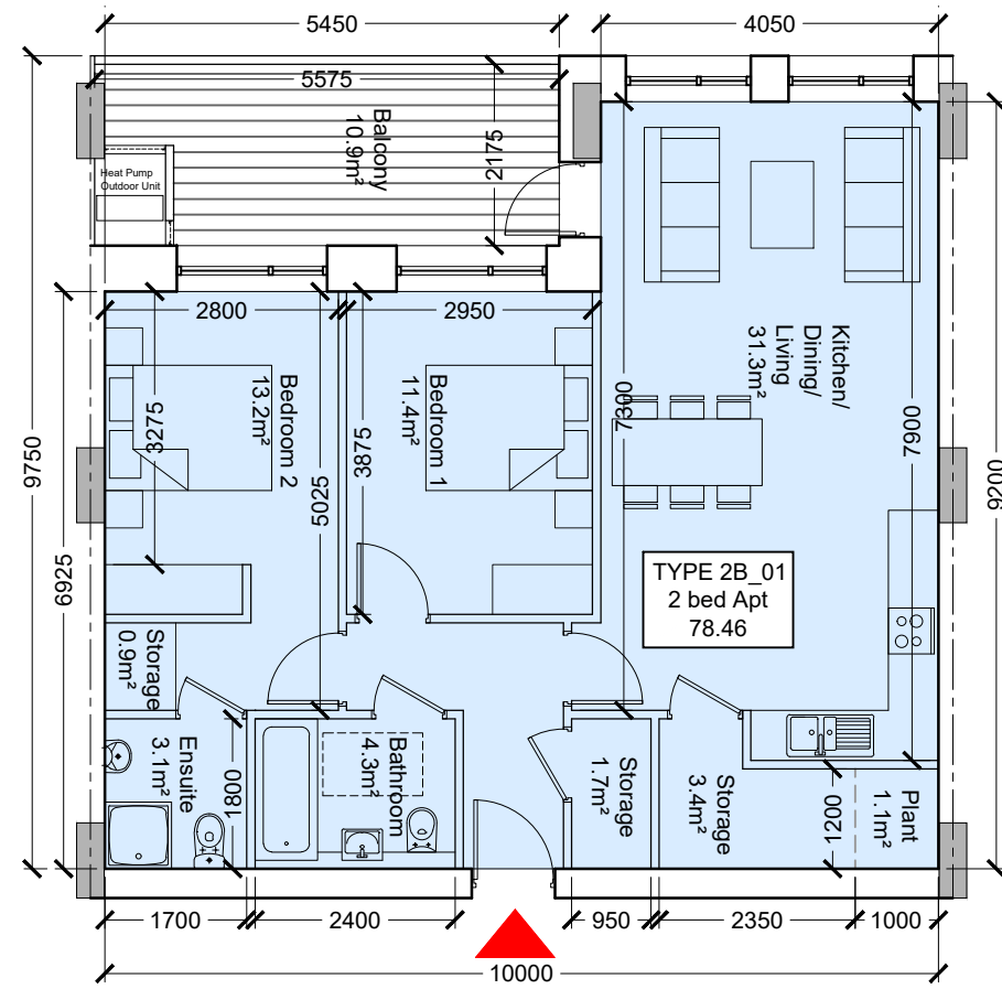
Type 2B_01 Scale 1:100
